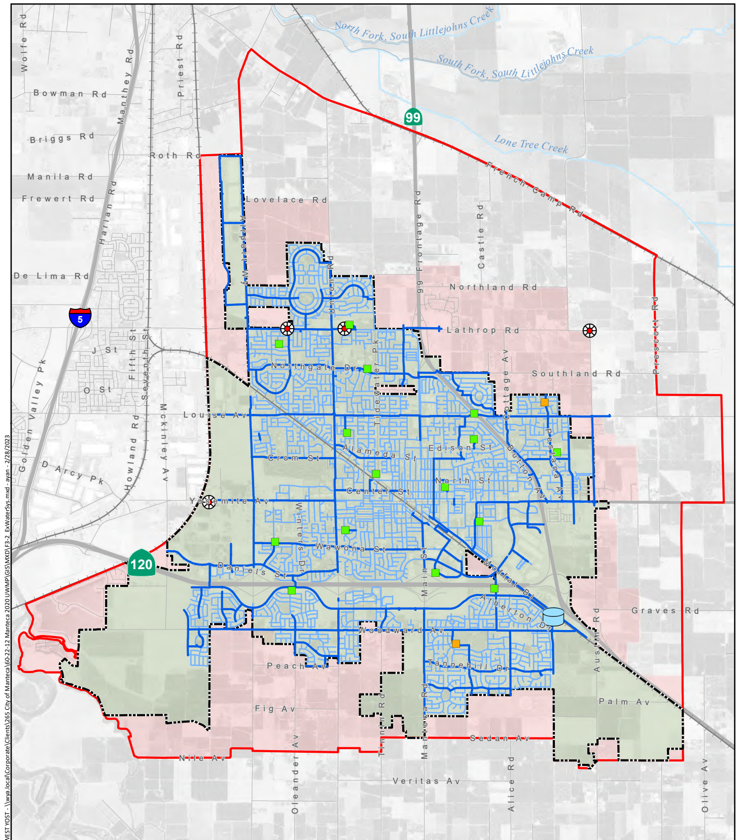
Figure 3-2 City of Manteca Existing Potable Water System
